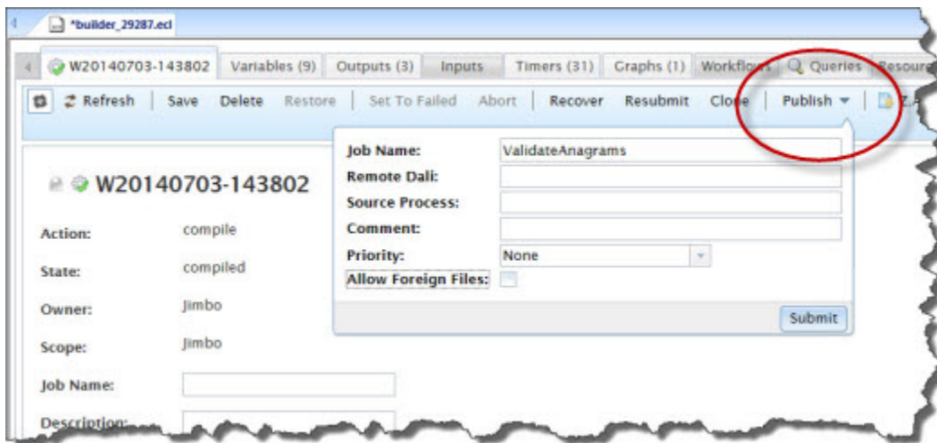
Figure 24. Publish Query
