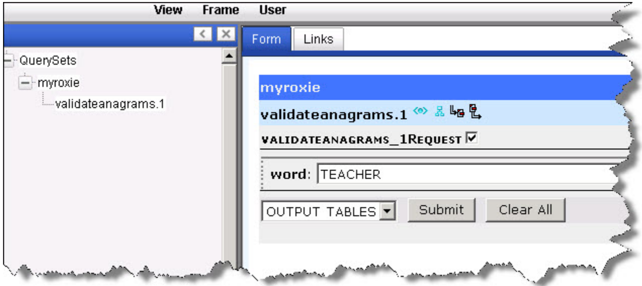
Figure 25. RoxieECL
