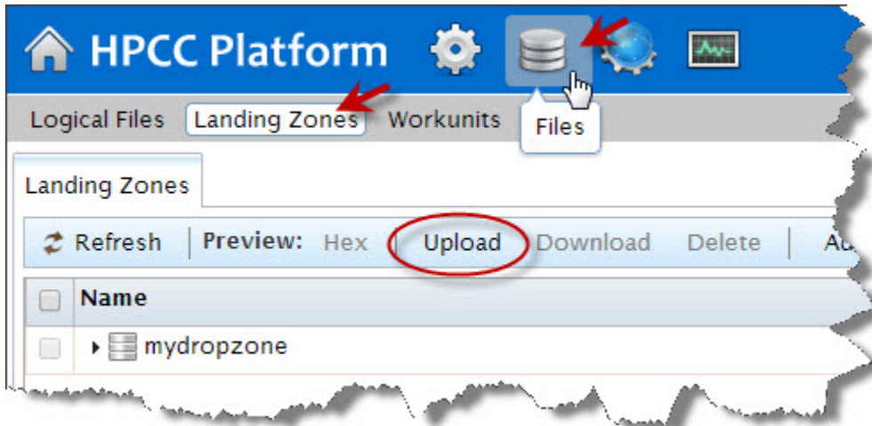
Figure 16. Upload
