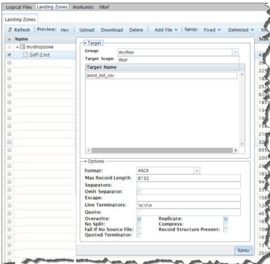
Figure 18. Spray Delimited
